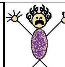
Oxygen
