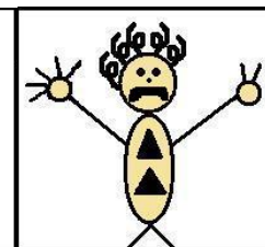
Nitrogen
