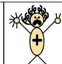
Fluorine
