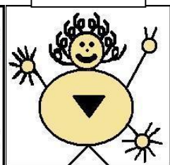
Argon
