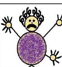
Sulfur
