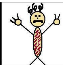
Boron
