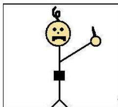
Hydrogen
