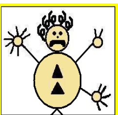
Phosphorus
