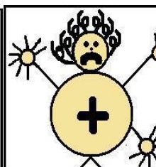
Chlorine
