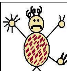
Aluminum
