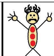
Carbon
