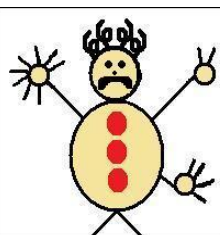
Silicon
