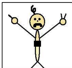
Lithium
