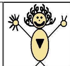
Neon
