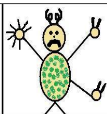
Magnesium
